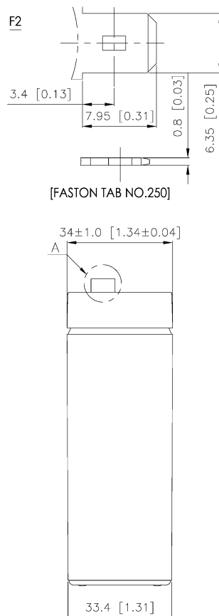
Detail A Drawing(3:1)
