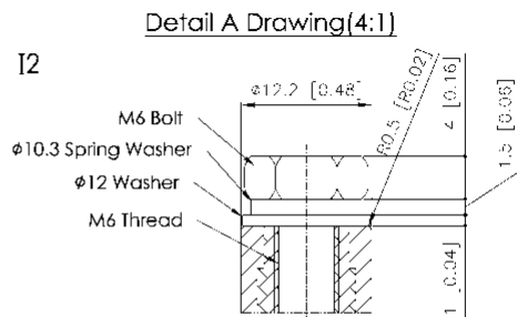
[M6 Bolt & M6 Thread & Washer & Spring Washer]
