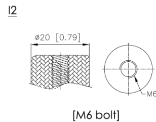
Detail A Drawing(4:1)
