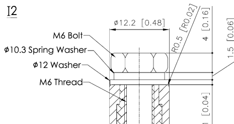
[M6 Bolt & M6 Thread & Washer & Spring Washer]
