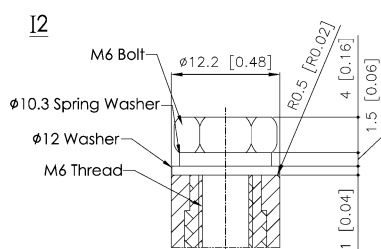
[M6 Bolt & M6 Thread & Washer & Spring Washer]
