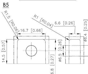
Detail A Drawing(3:1)
