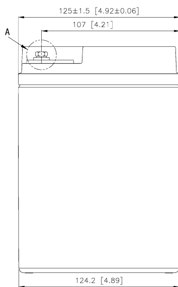
[M5 Bolt & M5 Thread & Spring Washer]
