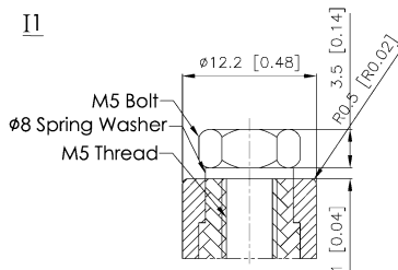
Detail A Drawing (4:1)
