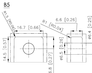
Detail A Drawing(3:1)
